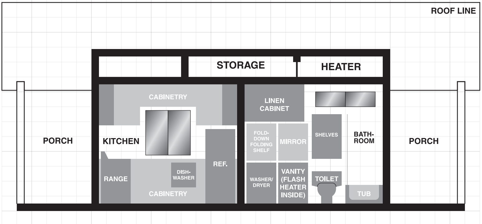
SECTION B-B
